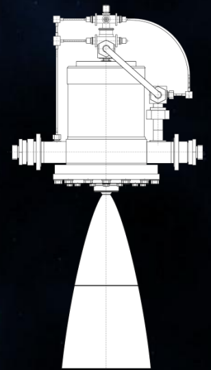
The "cold" reusable liquid rocket engine
